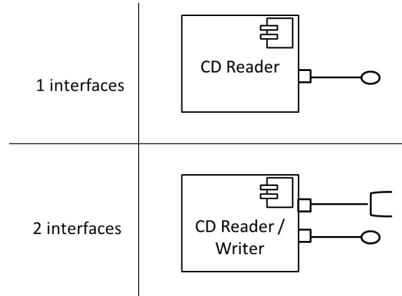
Figure 5.5: An instance of interface variability
