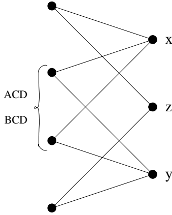
FIGURE 3.11 – \{T_2, T_3\} = \{ACD, BCD\}
