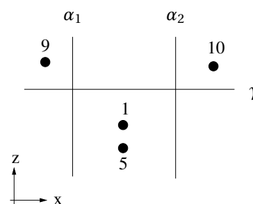
FIGURE 3.6 – View from below
