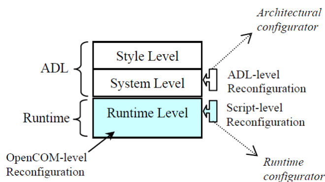
FIGURE 3.3: The architecture of Plastik [Joolia et al., 2005]
