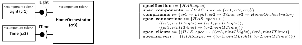
FIGURE 6.9: HAS specification
