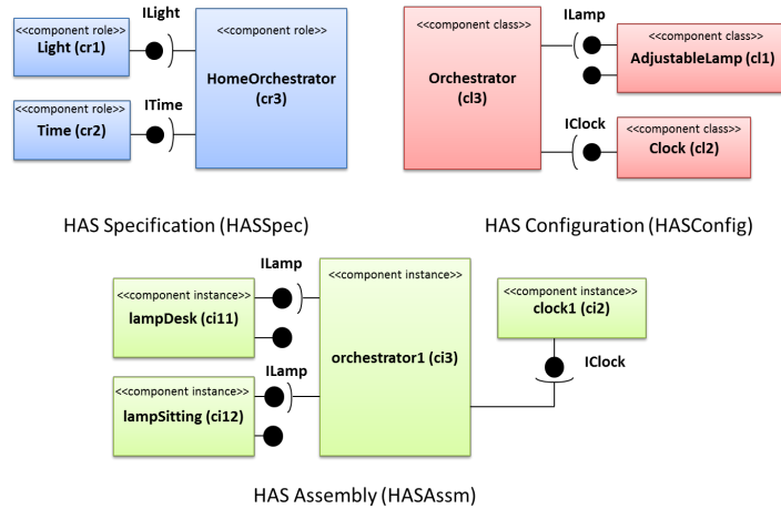
FIGURE 4.3: The architecture descriptions of HAS
