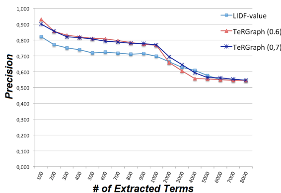
Figure 6.6: Precision comparison of LIDF-value and TeRGraph
