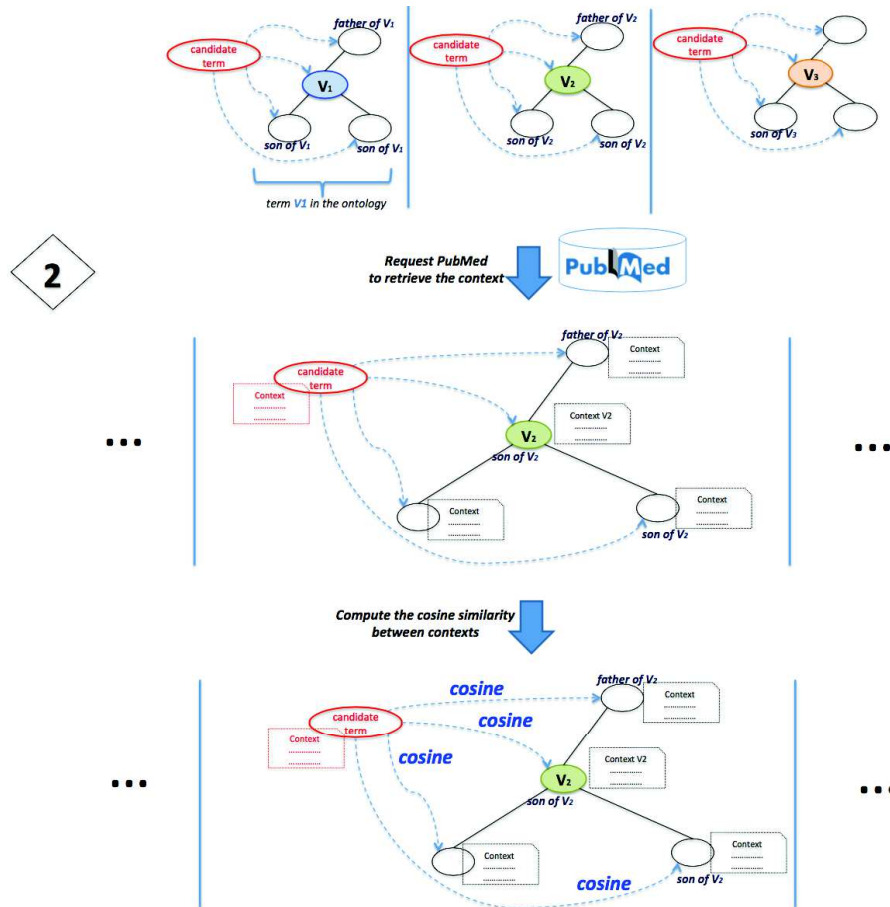
Figure 11.11: Second Semantic Linkage step.
