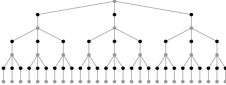
Figure 4.4: A worst-case associated dialogue tree with k = 3 . Gray-colored nodes are support move nodes while black-colored nodes are counter move nodes.
