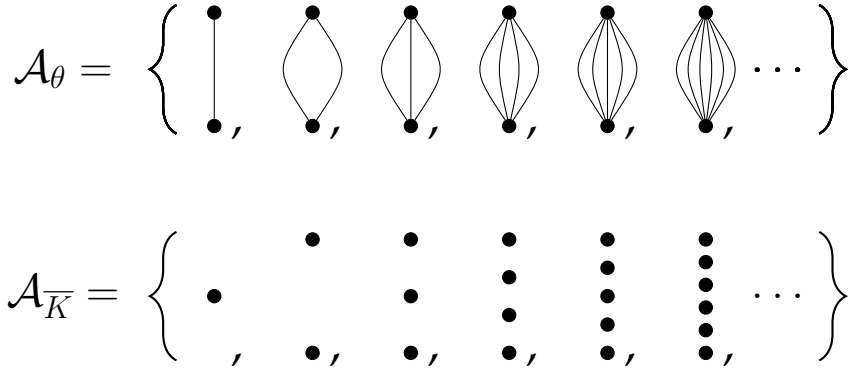
Figure 3.25: Two infinite antichains for multigraph contractions: multiedges and edgeless graphs.
