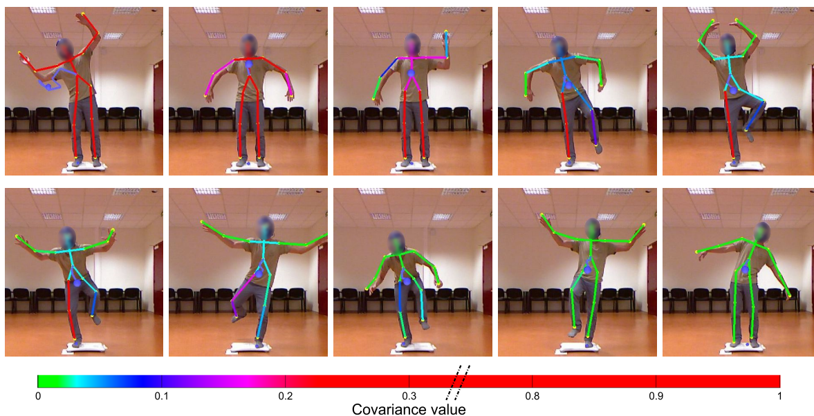
FIGURE 6.4: Adaptive interface for personalized center of mass estimation: The skeleton color changes from red to green indicating the convergence of the SESC model adaptively identified by the Kalman filter. Each segment color is determined by its respective covariance, where the highest value corresponds to red. The current CoM is also visible. We observe a high estimation error for the first frames and the CoM gradually entering the subject's body as the parameter identification proceeds. A video showing the identification procedure is available at http://youtu.be/J-yqOzRK5Ts .
