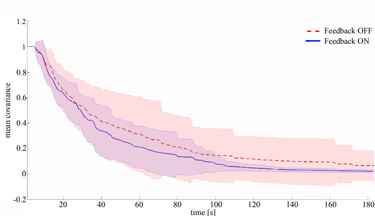
FIGURE 6.5: Mean and standard deviation of the maximum covariance among SESC parameters for all eight subjects during on-line identification. The red line shows the results without the adaptive interface while the blue line shows the results with the interface. The colored areas show the STD for each case. It is visible for the effects of the visual feedback on identification.
