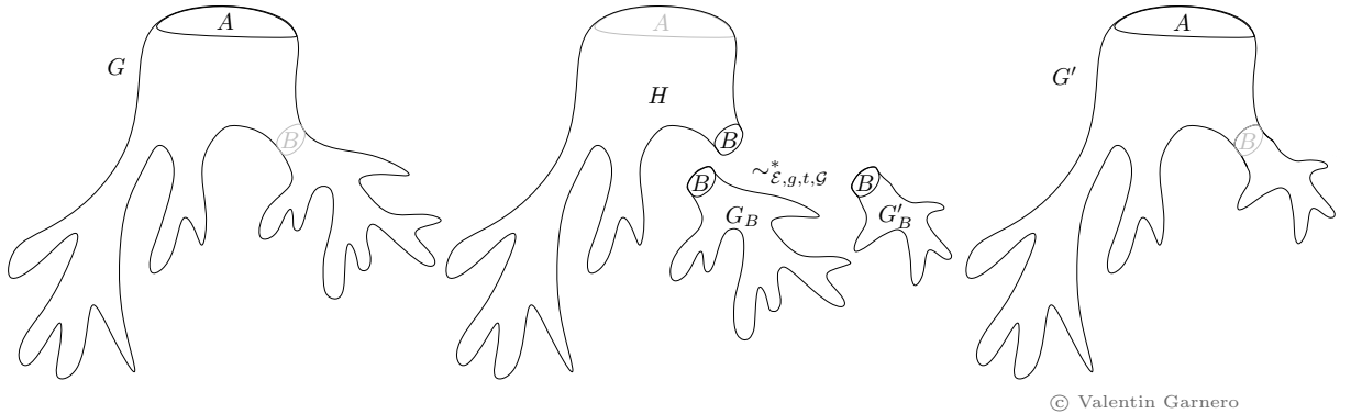
Figure 6.3: Graphs G and G' in the proof of Lemma 6.5.
