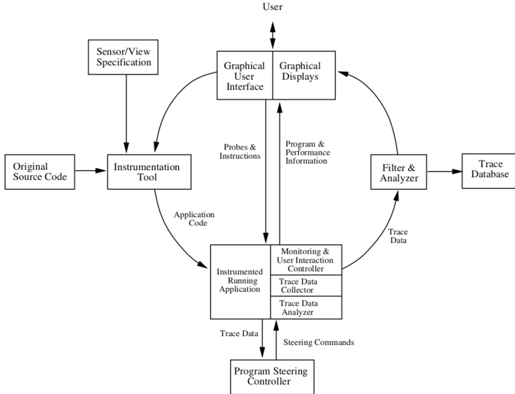
Figure 3.13: Falcon’s architecture [11].
