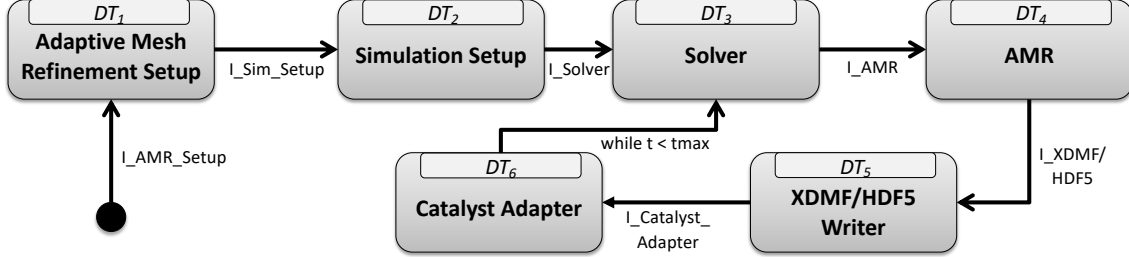
Figure 2.2: libMesh-sedimentation Workflow.
